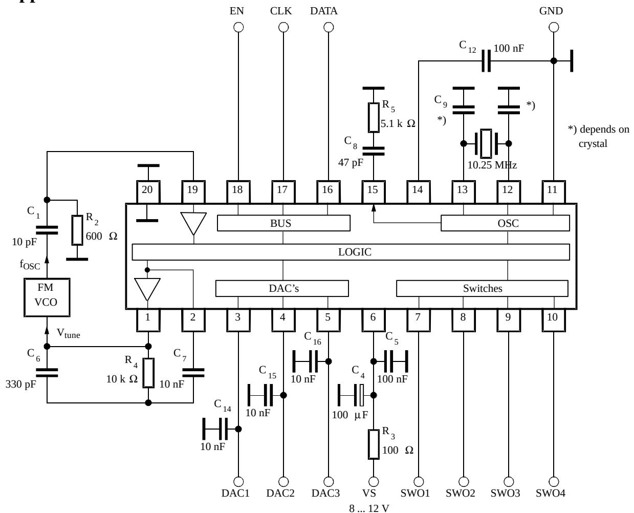
Figure 15. Application circuit
