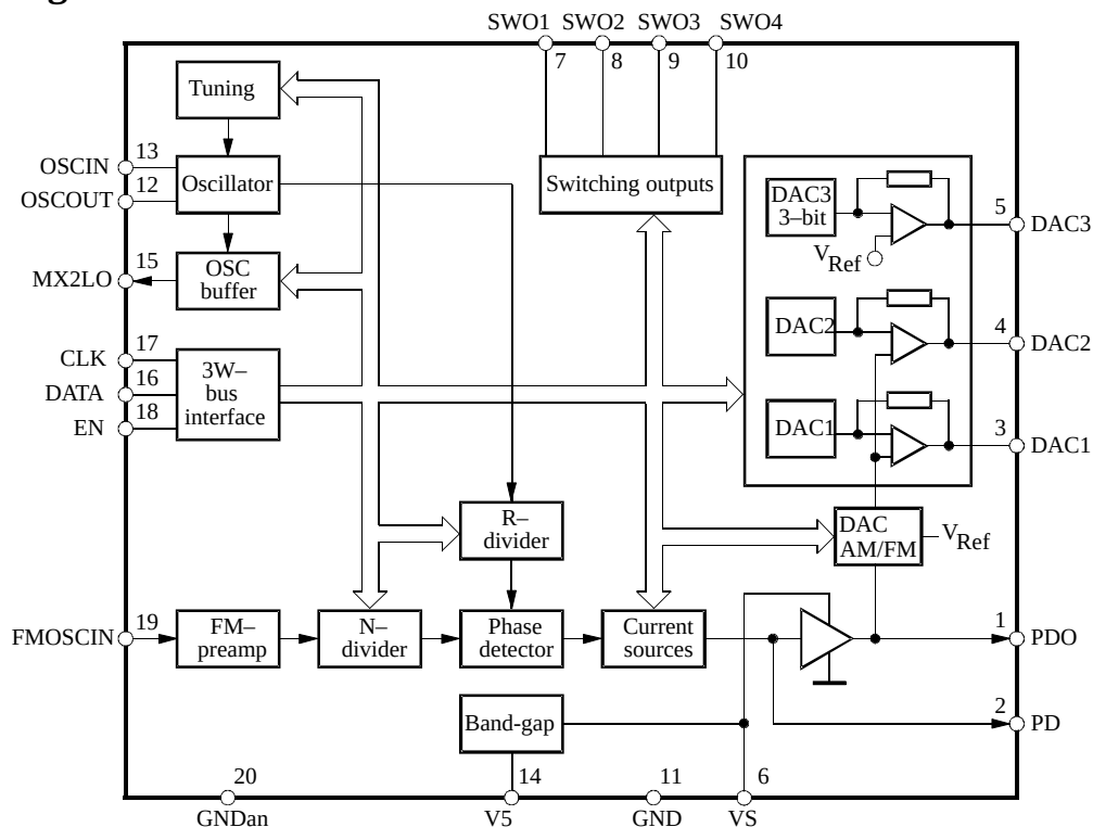
Figure 1. Block diagram
